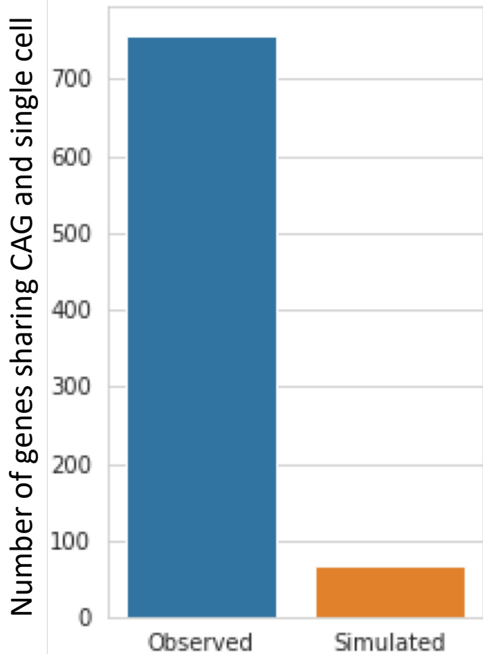
CRC-dataset generated CAGs
