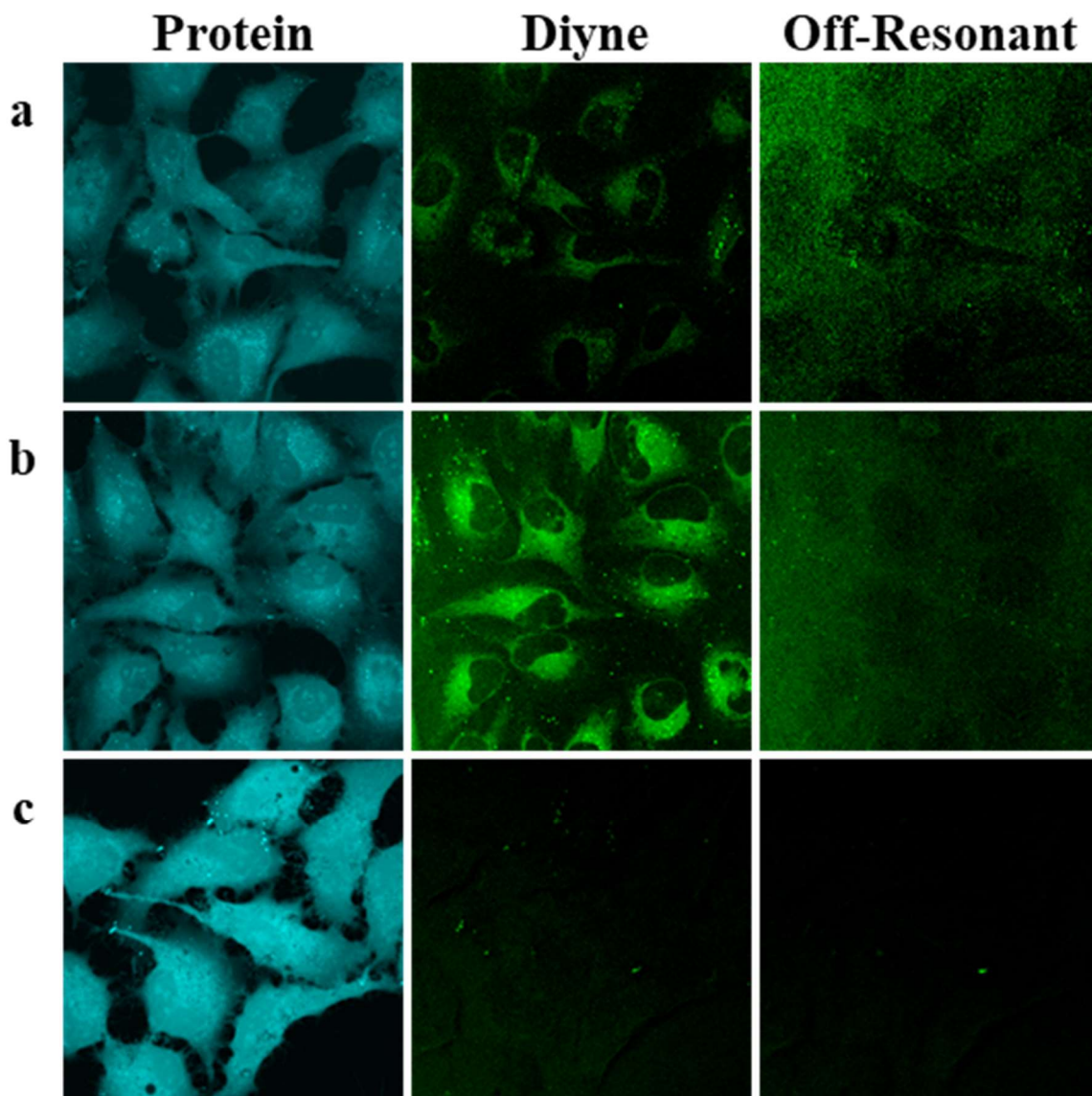
Figure S3. Intracellular PhDY-Ant ( 2 ) and phenyl-diyne tag imaging at various concentrations in HeLa cells. Cells were imaged 2h post PhDY-Ant addition at 10 \mu\text{M} (a) and 50 \mu\text{M} (b). Phenyl-diyne tag (50 \mu\text{M} ) was imaged as a negative control (c). SRS images were acquired by tuning the frequency difference between the pump and Stokes lasers to be resonant with protein ( \text{CH}_3 , 2940 \text{cm}^{-1} ), diyne (2251 \text{cm}^{-1} ), off-resonance (2000 \text{cm}^{-1} ).
