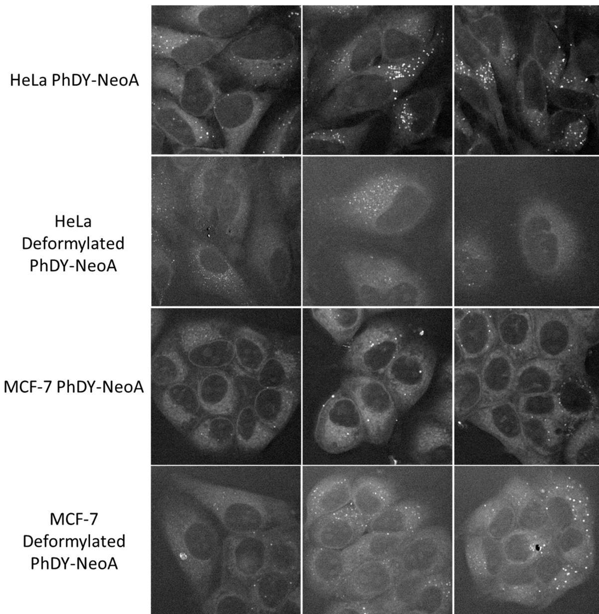
Figure S15. Imaging of differential uptake of PhDY-NeoA ( 4 ) and deformed PhDY-NeoA ( 6 ) in HeLa and MCF-7 cells. Raman imaging was performed using the diyne channel at 2251\text{ cm}^{-1} . Four different sets of Raman images are shown in triplicate.
