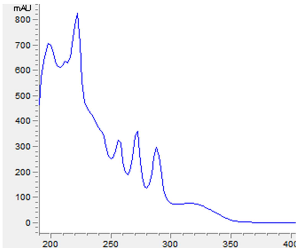
Figure S1: D) UV-vis spectrum of 2 .
