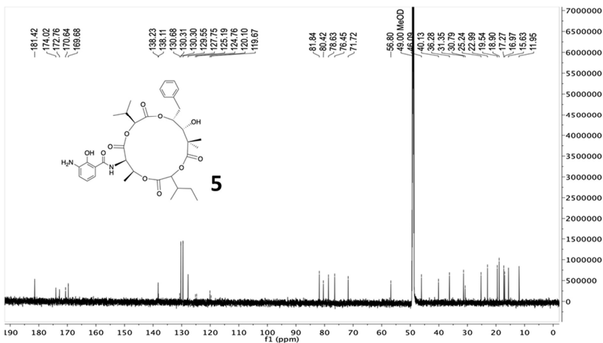
Figure S13. B) 13 C NMR spectrum (CD 3 OD, 226 MHz) of 5 .
