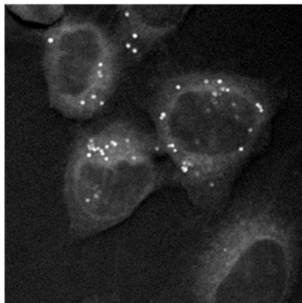
Figure S6. Temperature dependent uptake of PhDY-Ant ( 2 ). SRS images showing uptake of 50 \mu\text{M} 2 during 2h incubation at 4°C and 37 °C. 2 was still absorbed into HeLa cells at 4°C, indicating that the uptake mechanism is energy-independent.
