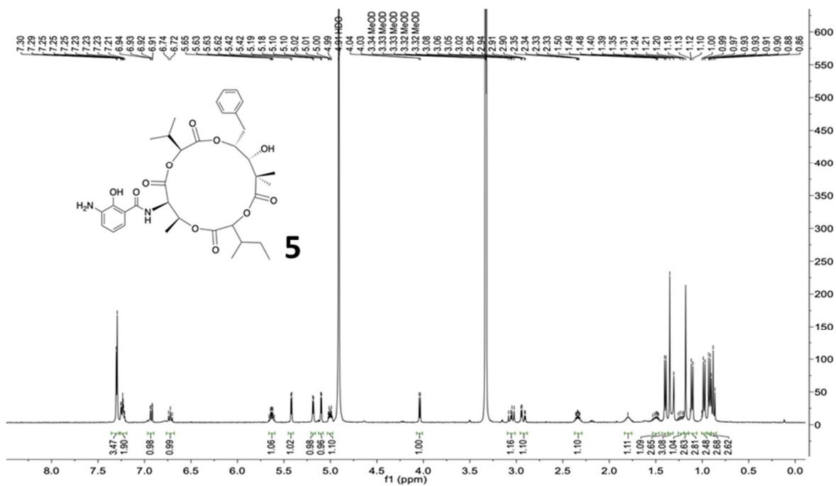
Figure S13. NMR, MS, and UV-vis characterization of deformylated neoantimycin ( 5 ). A) 1 H NMR spectrum (CD 3 OD, 900 MHz) of 5 .
