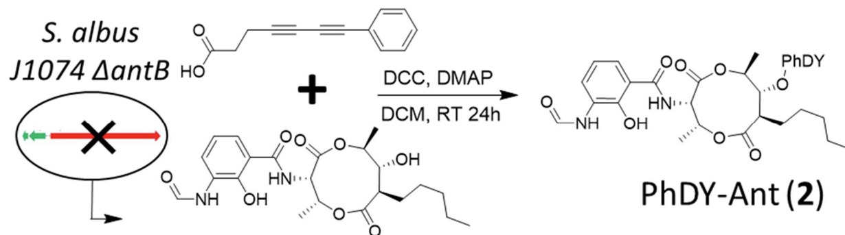
Scheme S1. Generation of PhDY-Ant (2) through both bioengineering and chemical derivatization.
