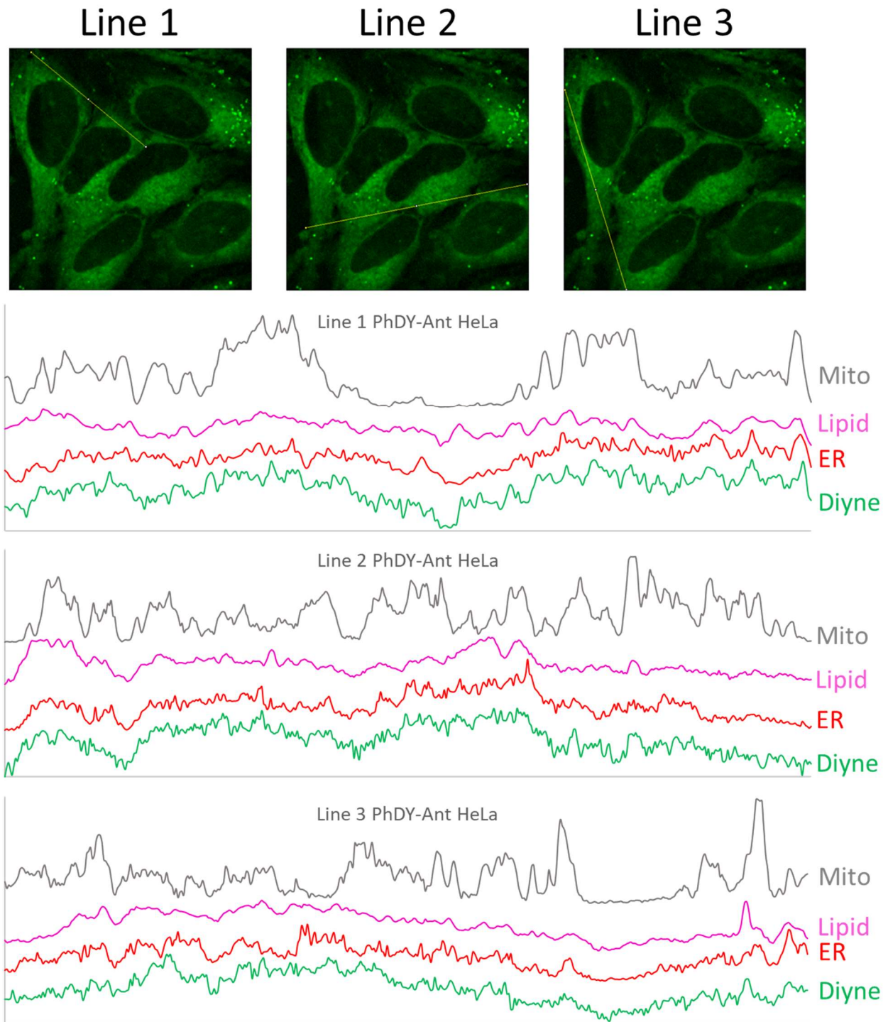
Figure S8. Line plot analysis of PhDY-Ant ( 2 ) in HeLa cells. Each line plot shows poor correlation between Mito-tracker and the diyne channel. Each line plot shows good correlation between the lipid channel and the diyne channel. The ER-tracker and diyne channels are very well-correlated, including some features that are excluded on the lipid channel.
