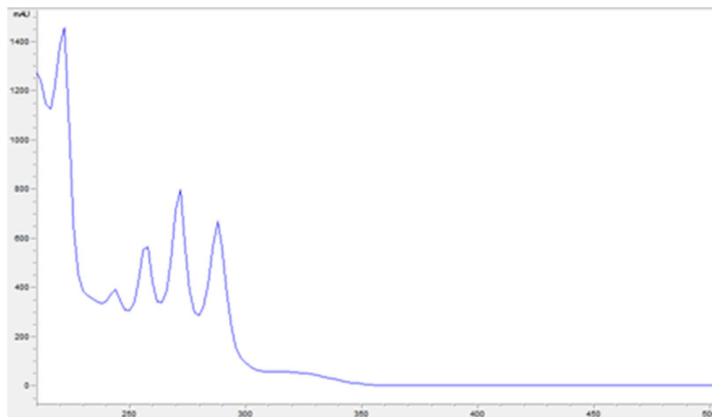
Figure S11. D) UV-vis spectrum of 4.
