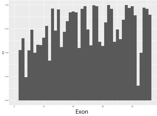
E PKD1 Proportion of bases covered >15 times
