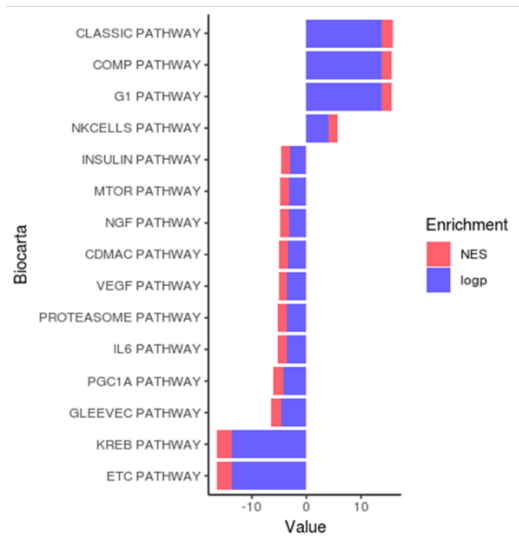
Supplemental Figure 10
