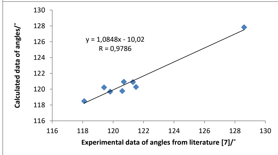
Figure S1. The correlation between calculated and literature data of bonds lengths and angles
