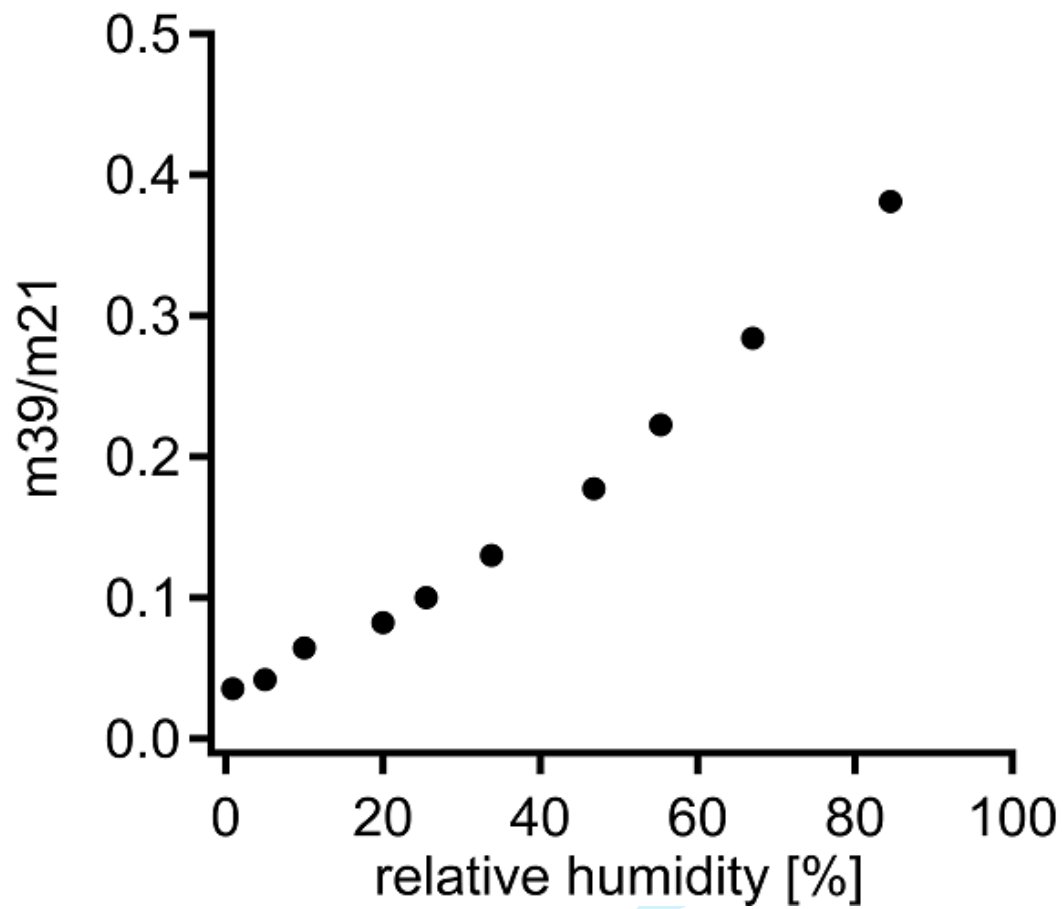
Figure S1. Relationship between the m39/m21-ratio and the relative humidity in %.
