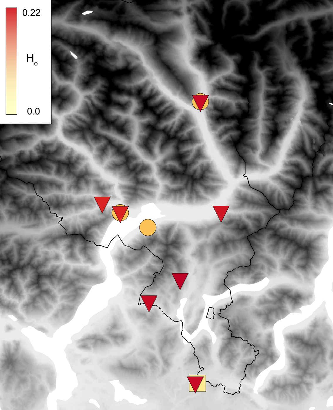
Fig. S1: Average heterozygosity of Pelophylax populations from Ticino, based on 2,521 SNPs. Circles: P. lessonae ; triangles: P. kl. esculentus ; square: P. ridibundus
