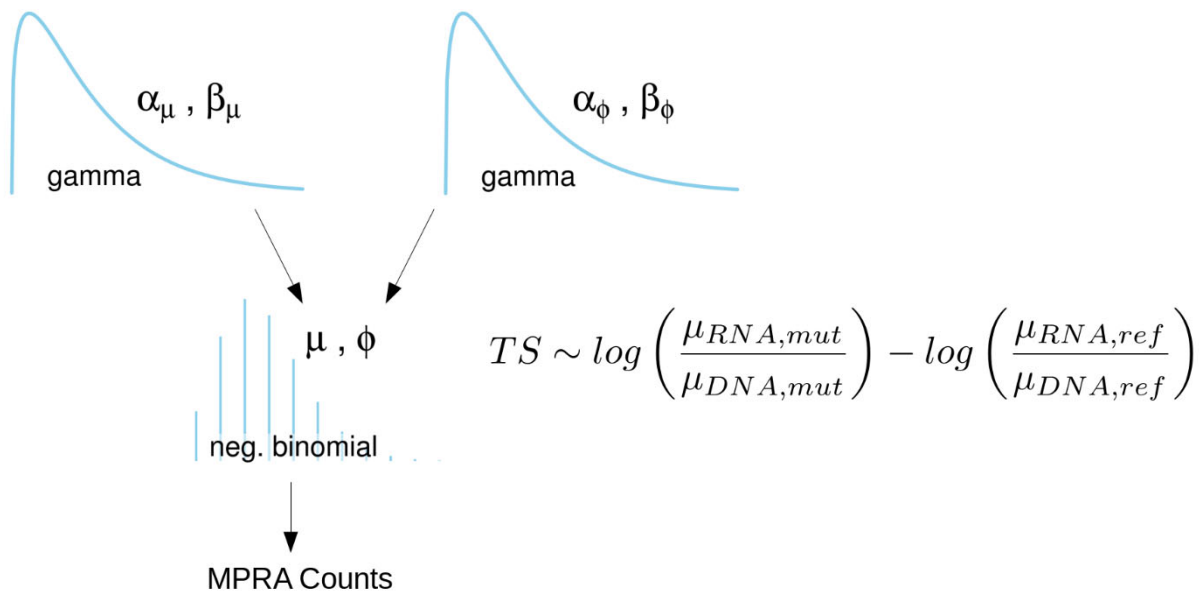
Figure S4 – Kruschke diagram showing the generative model underlying the Bayesian analysis. The mean parameters for the separate alleles and nucleic acids are aggregated after fitting the model into a posterior on transcription shift that is used to identify functional SNPs.
