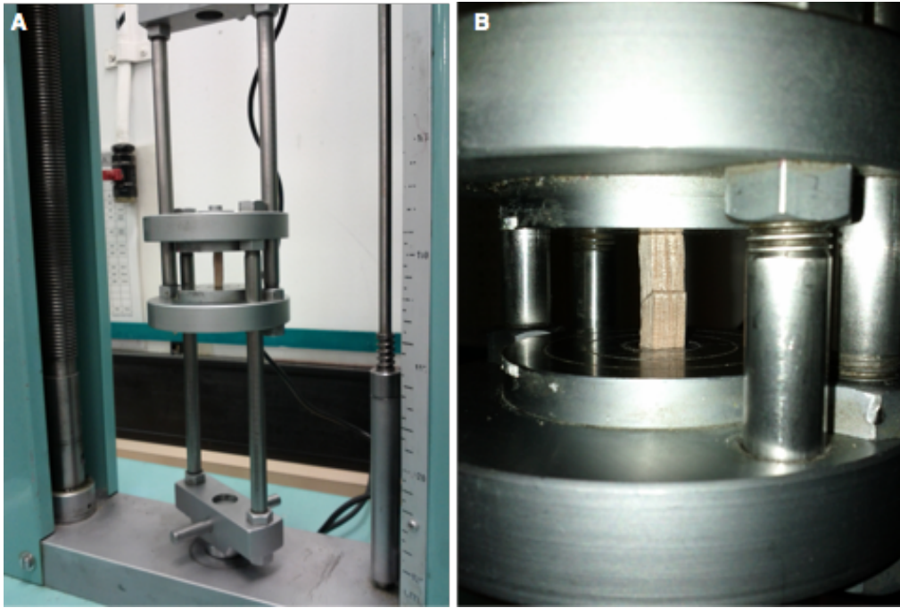
Fig. S3. Quasi-static compression test, A , experimental setup, B , close-up of sample after the point of yielding strength being crushed with clearly visible slip plane.
