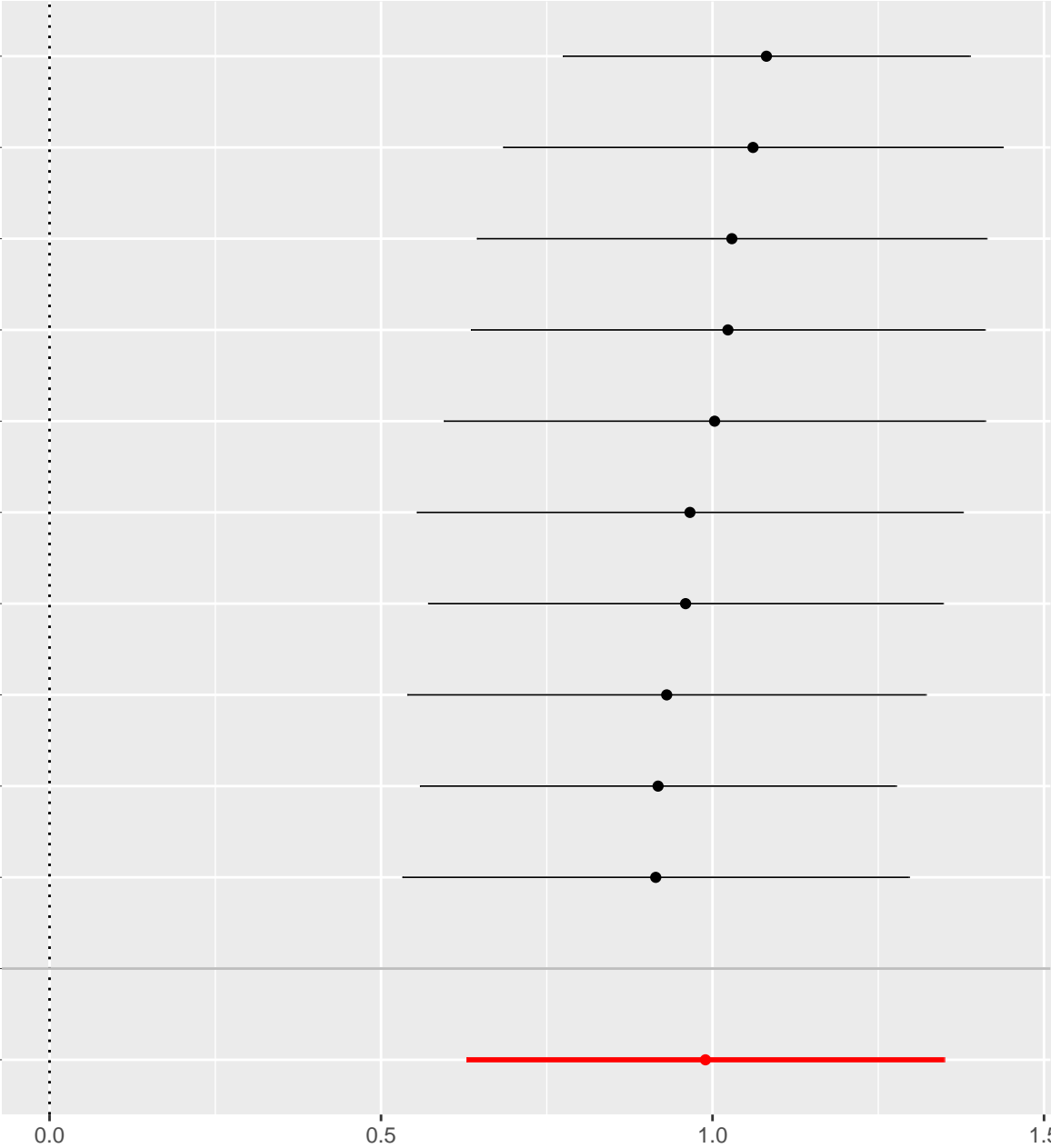
MR leave-one-out sensitivity analysis for 'Genetic liability to endometriosis' on 'Clear cell ovarian cancer'
