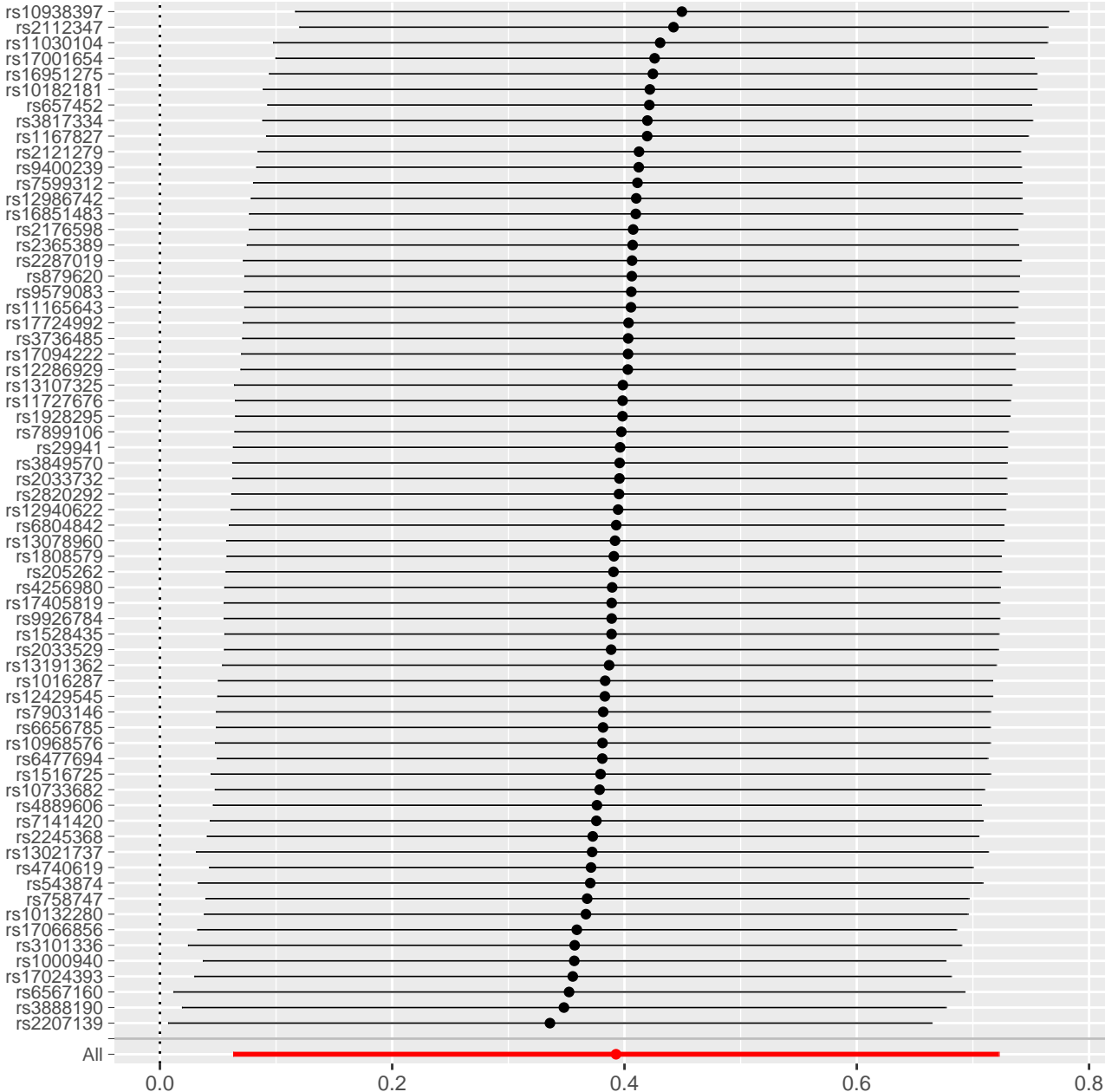
MR leave-one-out sensitivity analysis for 'Body mass index' on 'Endometrioid ovarian cancer'
