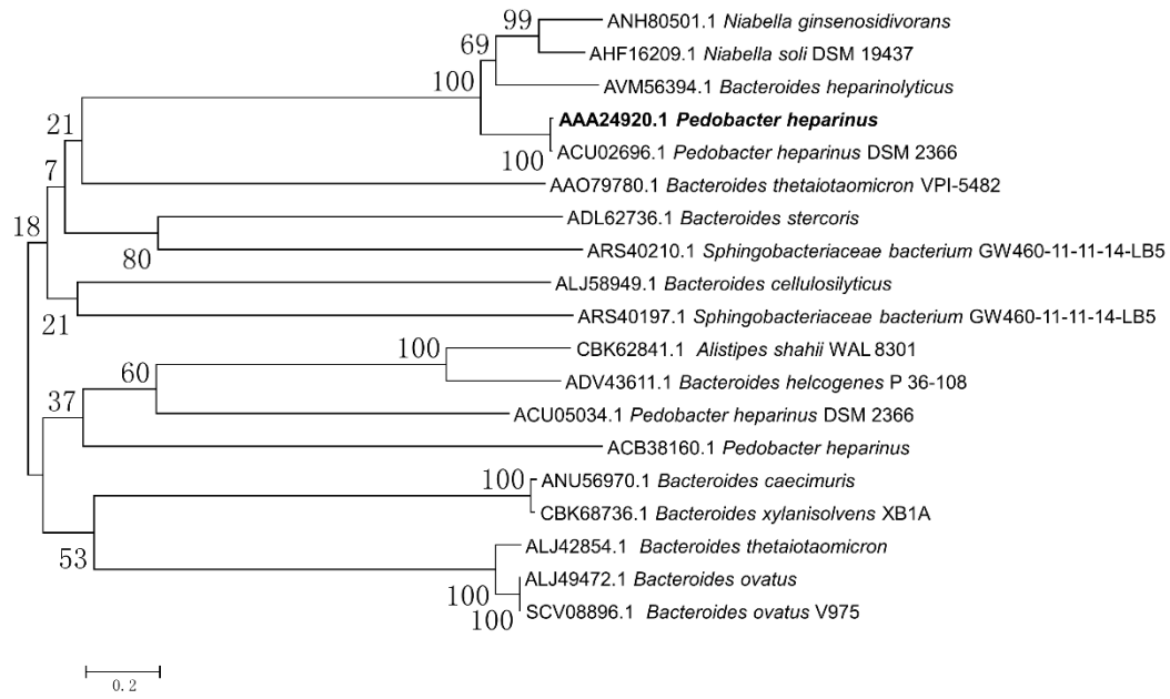
Figure S1 Phylogenetic tree of characterized heparinase I of PL13 family.
