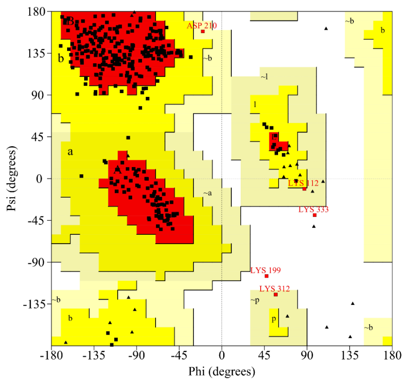
Figure S2 The stereochemical spatial arrangement of amino acid residues in the modeled 3D structure of Ph-HepI in favored region of the Ramachandran plot.
