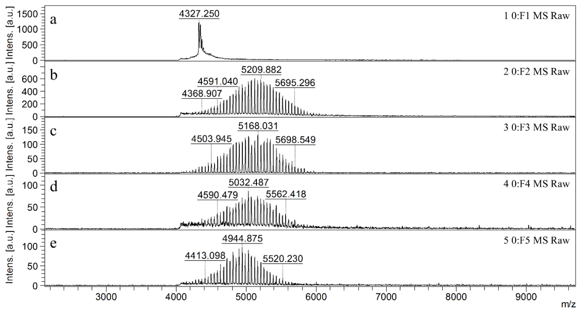
Figure S3 Mass spectrometry analysis of degradation products. (a) LMWH standard; (b) Degradation product of Wild-type enzyme; (c) Degradation product of mutant enzyme (S169D); (d) Degradation product of mutant enzyme (A259D); (e) Degradation product of mutant enzyme (S169D/A259D).
