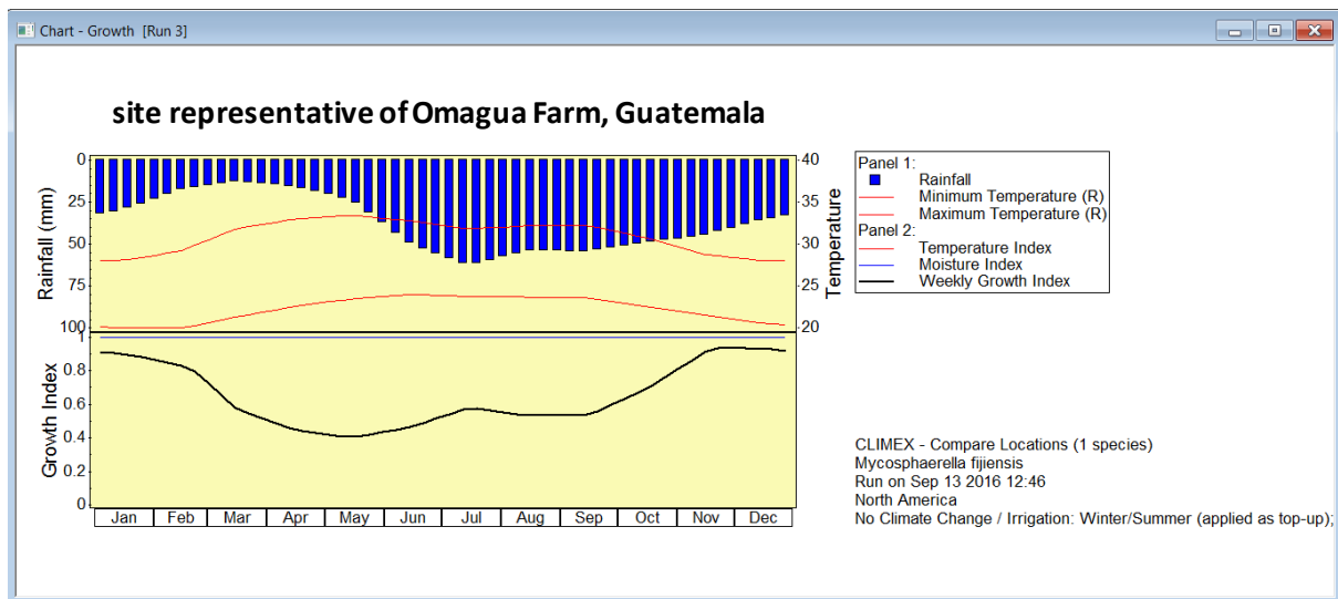
Fig S9. Growth chart for P. fijiensis in an area representative of Omagua Farm, Guatemala, and expert database site #72. Model was run with 5mm day -1 irrigation added as top-up. Growth is temperature-limited under this irrigation scenario.
