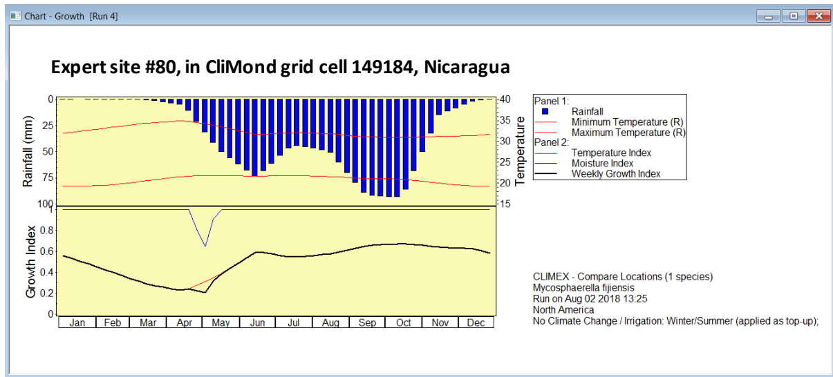
Fig S11. Growth chart for P. fijiensis at expert database site #80 in Nicaragua. Model was run with 5mm day -1 irrigation added as top-up.
