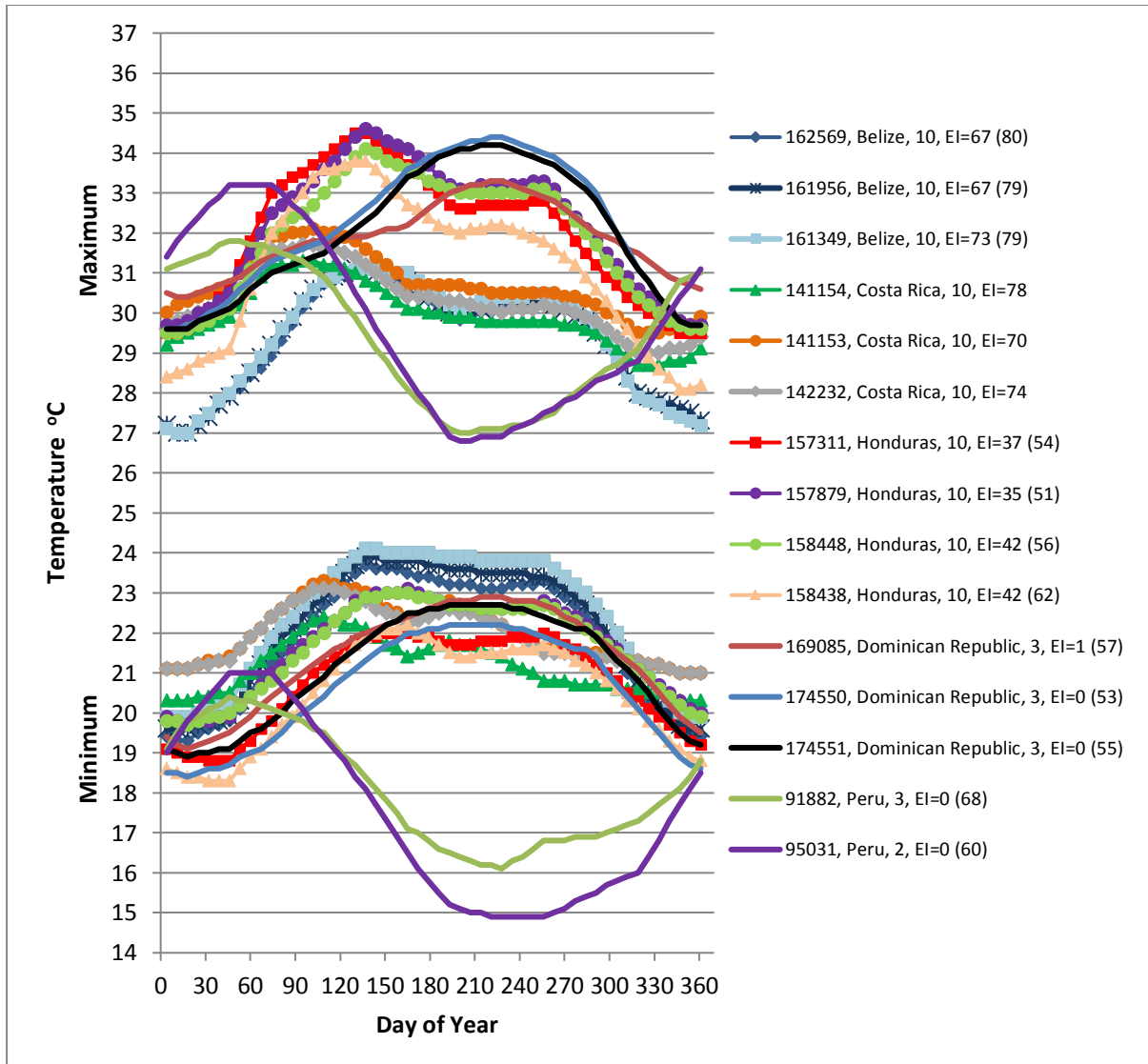
Fig S15. Minimum and maximum temperatures of the CLIMEX grid cells containing the ten highest-ranked locations (lines with markers) and the five lowest-ranked locations (solid lines, no markers) of P. fijiensis . For each location, grid cell number, country, disease pressure ranking, and EI value without irrigation (and with irrigation in brackets) are given.
