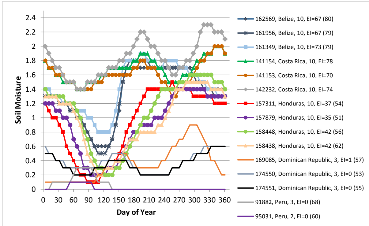
Fig S16. Soil moisture values of the CLIMEX grid cells containing the ten highest-ranked locations (lines with markers) and the five lowest-ranked locations (solid lines, no markers) of P. fijiensis . For each location, grid cell number, country, disease pressure ranking, and EI value without irrigation (and with irrigation in brackets) are given.
