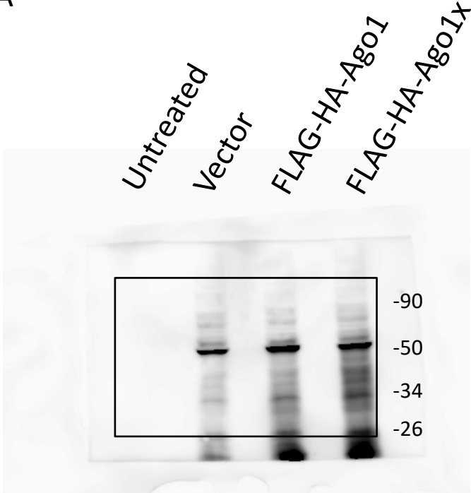
Anti- Puromycin
