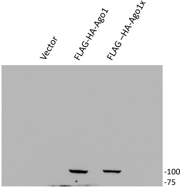
Anti-HA
