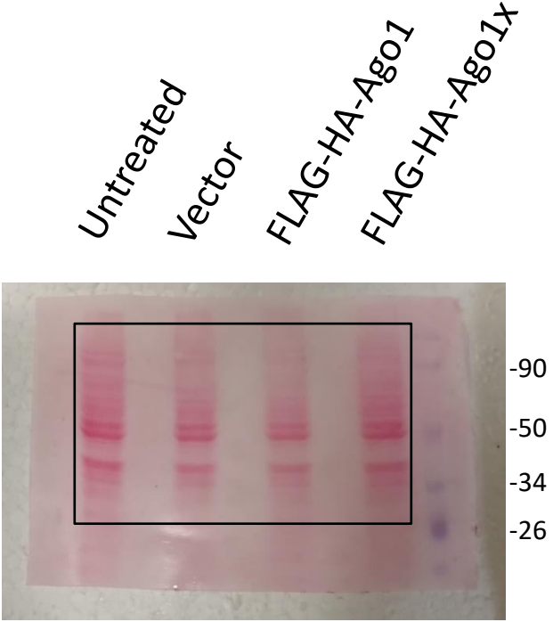
Ponceau S
