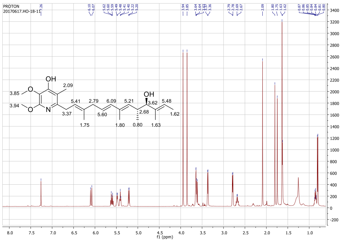
S4 Fig. 1 H NMR of piericidin-A 1 (2) (CDCl 3 , 500 MHz)
