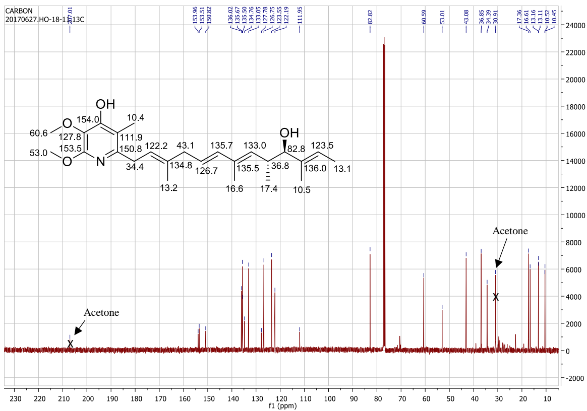
S5 Fig. 13 C NMR of piericidin-A 1 (2) (CDCl 3 , 125 MHz)
