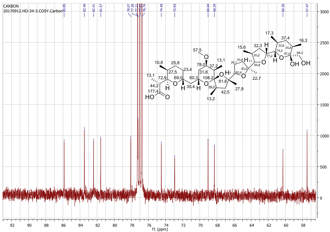
S10 Fig. ^{13}\text{C} NMR of nigericin ( 3 ) ( \text{CDCl}_3 , 125 MHz). Region of 56 to 110 ppm.
