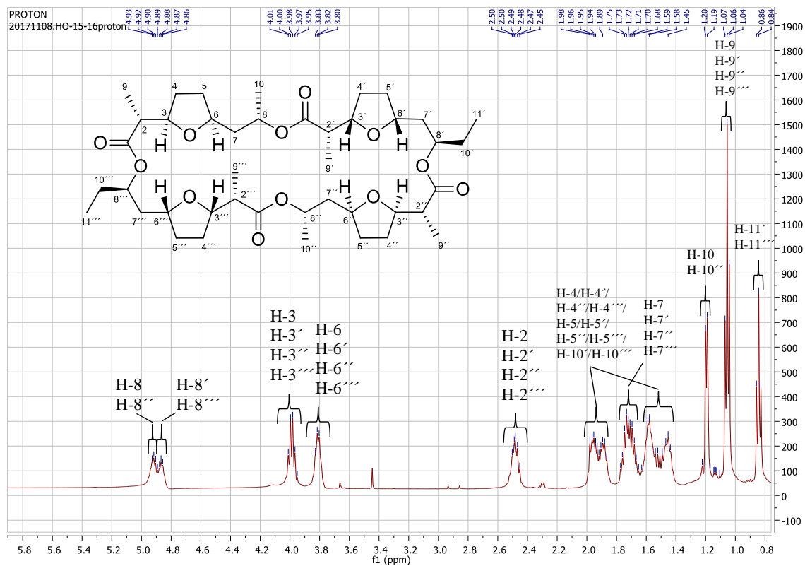
S12 Fig. ^1\text{H} NMR of dinactin ( 4 ) ( \text{CDCl}_3 , 500 MHz)
