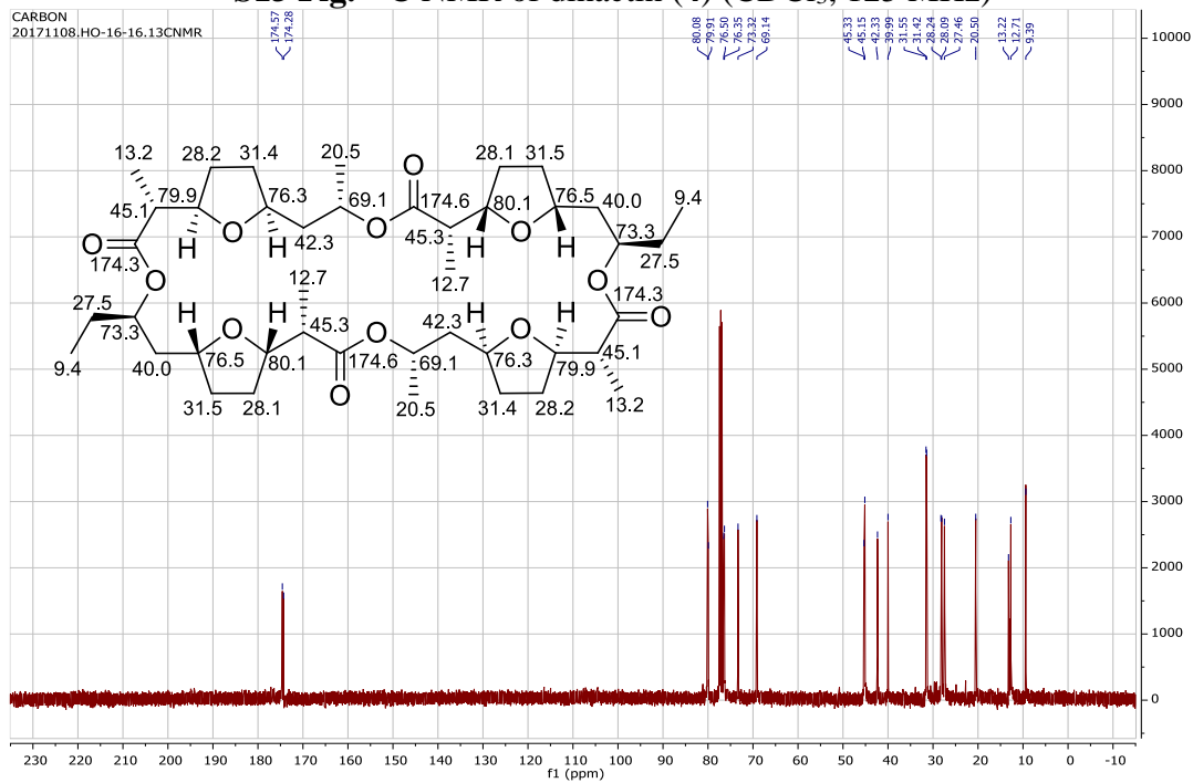
S13 Fig. ^{13}\text{C} NMR of dinactin ( 4 ) ( \text{CDCl}_3 , 125 MHz)
