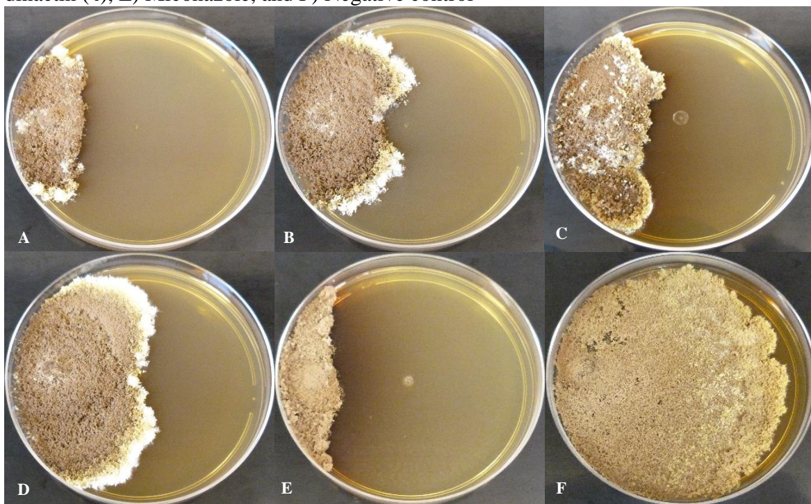
S16 Fig. Antagonist activity of compounds (100 \mu g) against Escovopsis sp ICBG740 (21 days of growth at 28 °C): A) Mer-A2026B (1), B) piericidin-A 1 (2), C) nigericin (3), D) dinactin (4), E) Miconazole, and F) Negative control
