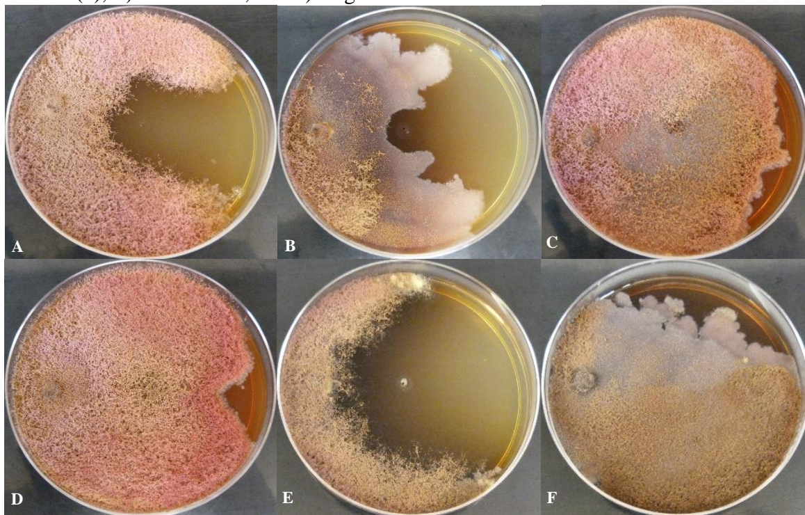
S17 Fig. Antagonist activity of compounds (100 \mu g) against Escovopsis sp ICBG1251 (21 days of growth at 28 °C): A) Mer-A2026B ( 10 ), B) piericidin-A 1 ( 11 ), C) nigericin ( 12 ), D) dinactin ( 4 ), E) Miconazole, and F) Negative control
