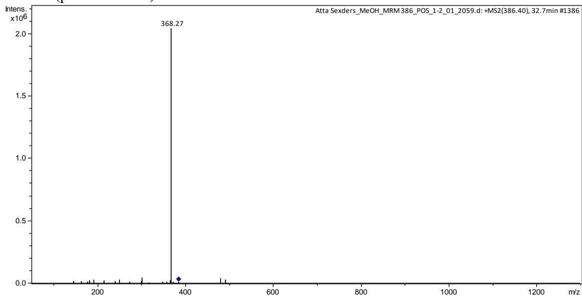
S19 Fig. MS/MS spectra of compound eluted at 32.7 minutes ( m/z 386.40), identified as mer-A2026B (positive mode)
