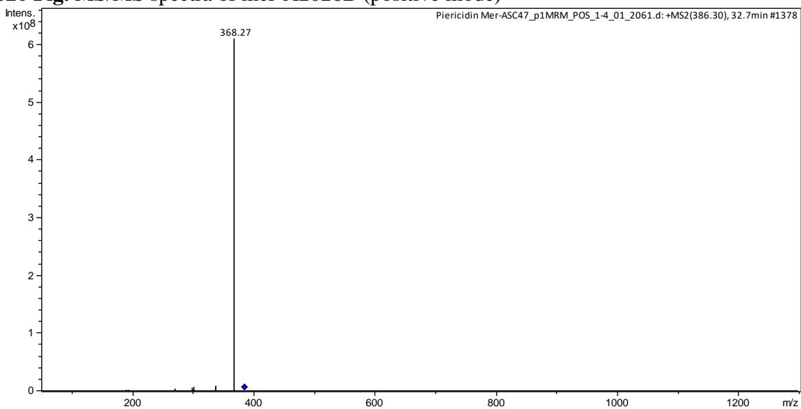
S20 Fig. MS/MS spectra of mer-A2026B (positive mode)
