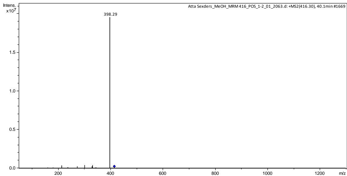
S22 Fig. MS/MS spectra of compound eluted at 40.1 minutes ( m/z 416.30), identified as piericidin A (positive mode)
