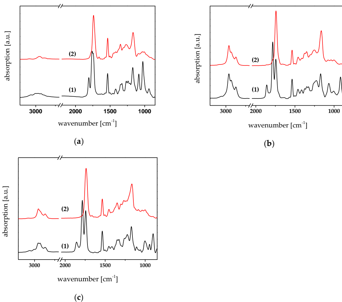
Figure S1. FT-IR spectra of (a) epoxy-NBE/GA, (b) epoxy-NBE/DDSA and (c) epoxy-NBE/HHMPA (1) prior to and (2) after thermal curing at 100 °C.
