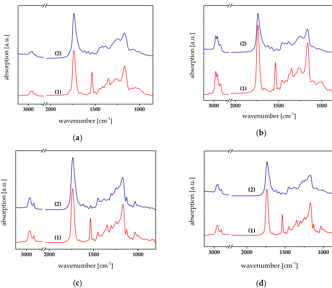
Figure S2. FT-IR spectra of (a) epoxy-NBE/GA, (b) epoxy-NBE/DDSA and (c) epoxy-NBE/HHMPA (1) prior to and (2) after photocleavage (74.5 mW cm -2 ).
