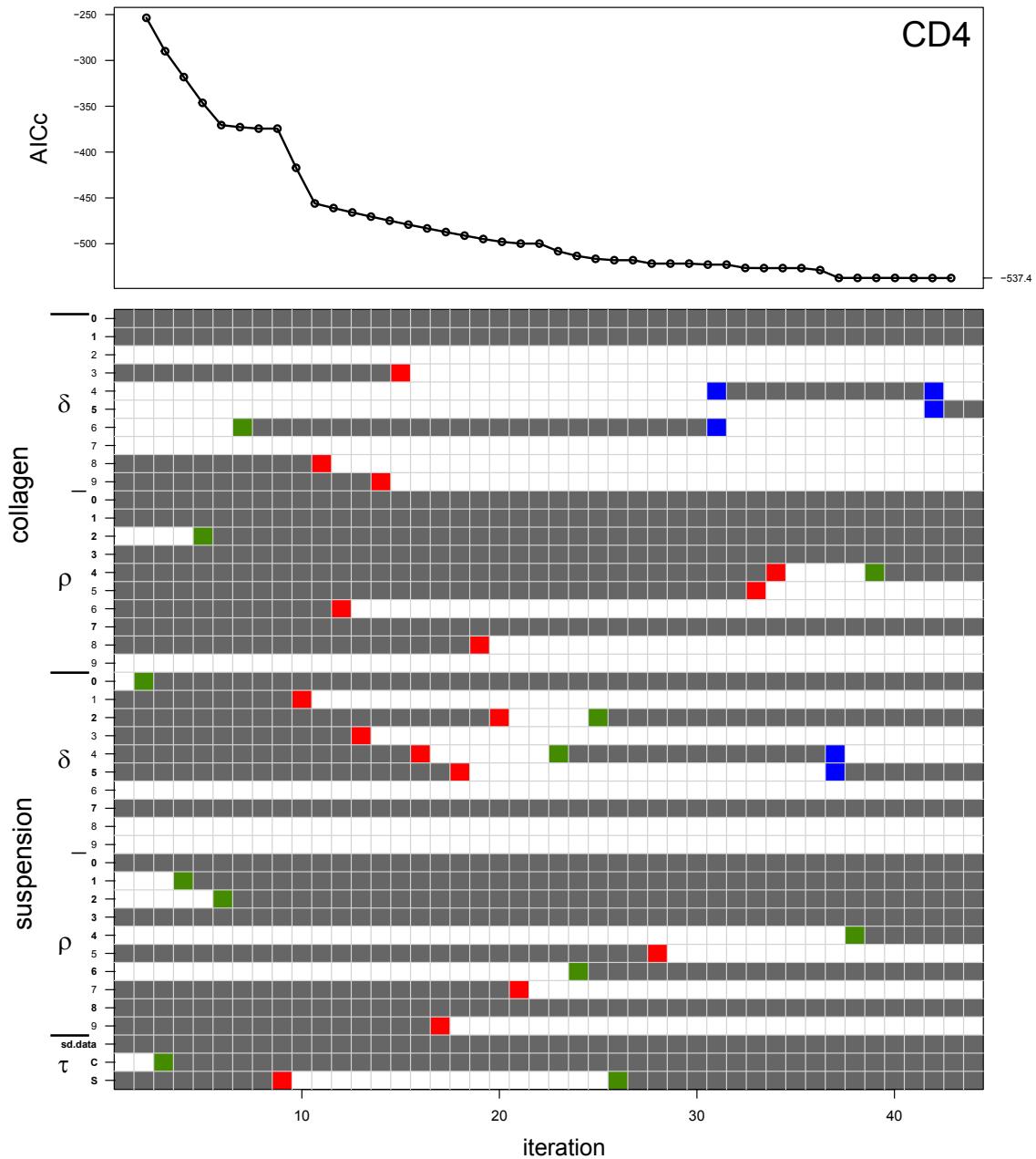
Figure S2: Exemplary FAMoS-run analysing CD4 + T cell dynamics: Visualization of a single FAMoS-run over several iterations with the addition ( forward search , green), removal ( backward elimination , red) and swapping ( swap search , blue) of parameters for analysing the turnover dynamics of CD4 + T cells in suspension and collagen. Parameters that are selected in the final model with the denoted AICc-value of -537.4 are indicated in bold. The final run out of 5 individual FAMoS runs is shown.
