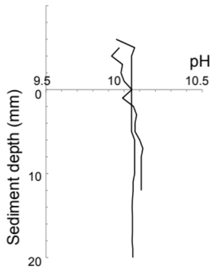
Figure S2 pH profile measured on two replicate sediment columns.
