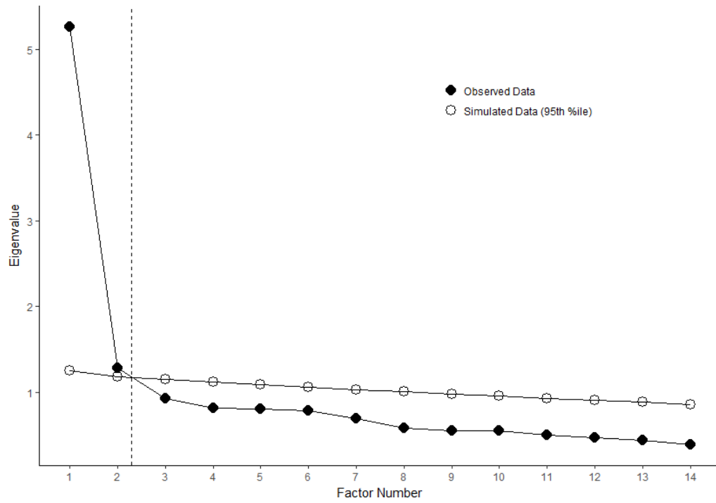
S1 Fig. Parallel analysis and eigenvalues of factor analysis.
