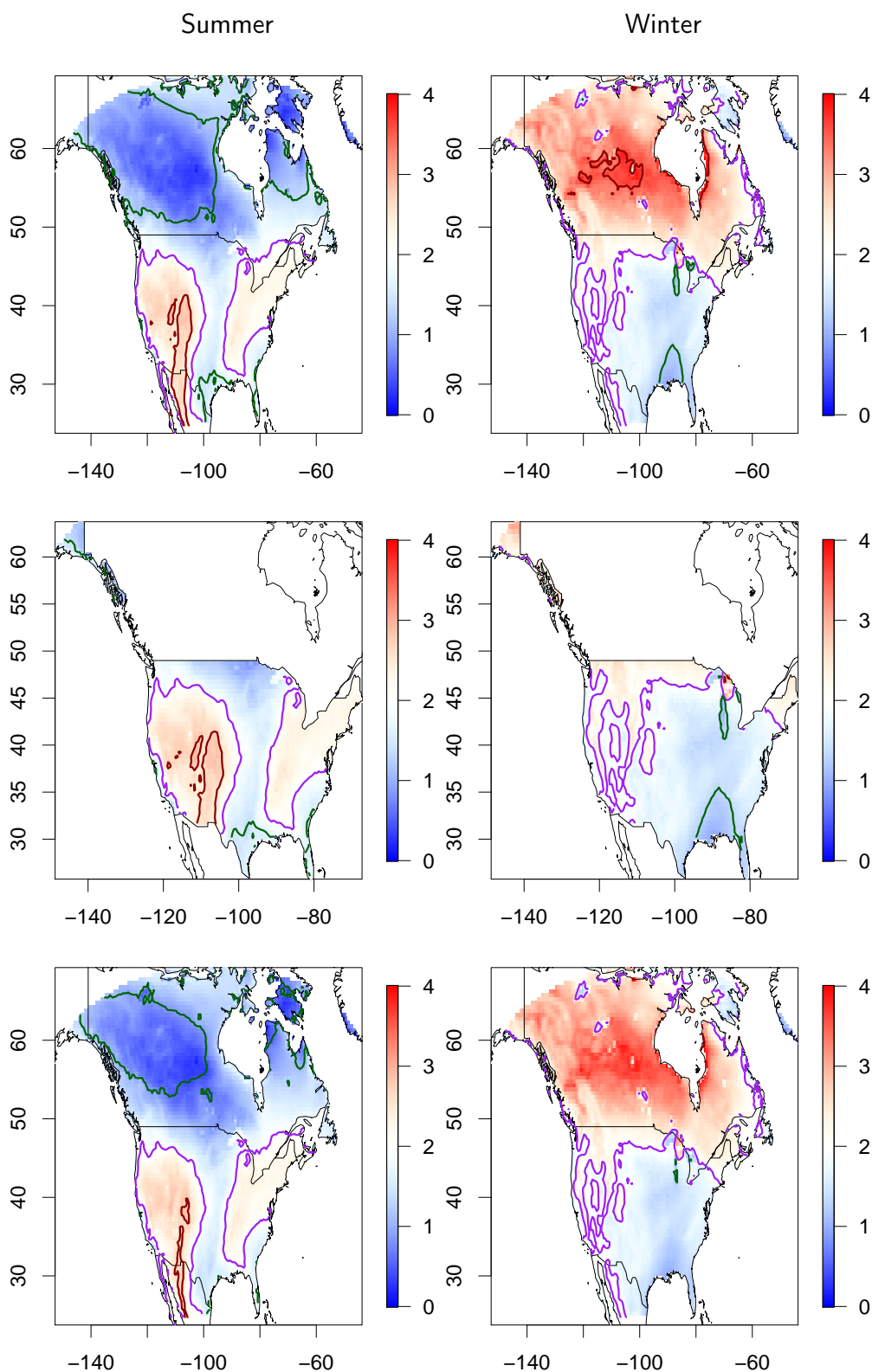
Figure 5: CoPE sets for entire domain (North America)(top row), US only (middle) and confidence regions for the excursion set A_c for c = 2^\circ C obtained via pixel-wise testing and Holm correction (bottom).
