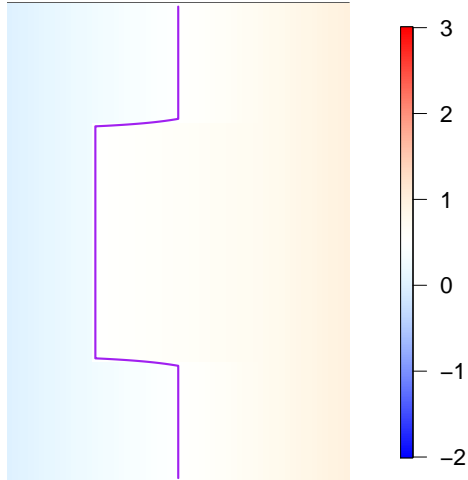
Figure 1: The discontinuous signal.
