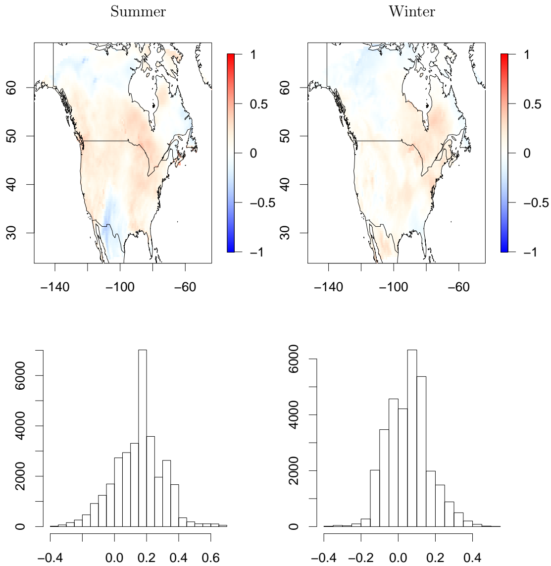
Figure 4: Estimated AR coefficients for the linear model fitted to the climate data: spatial distribution (top row) and histogram over locations (bottom row).
