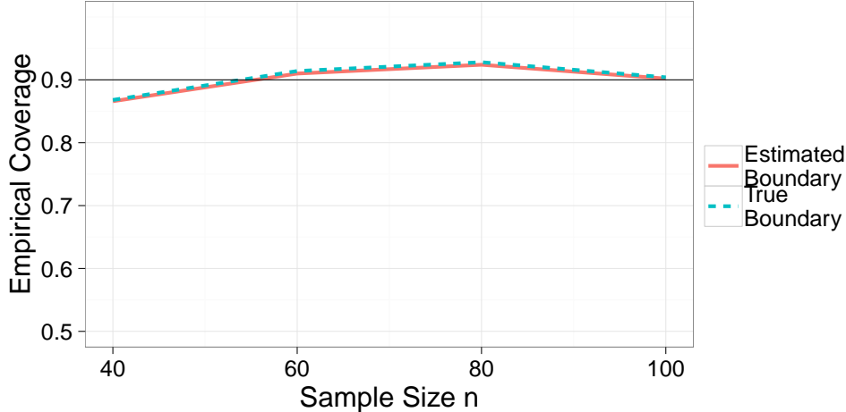
Figure 3: Empirical coverage of CoPE sets for the discontinuous signal.
