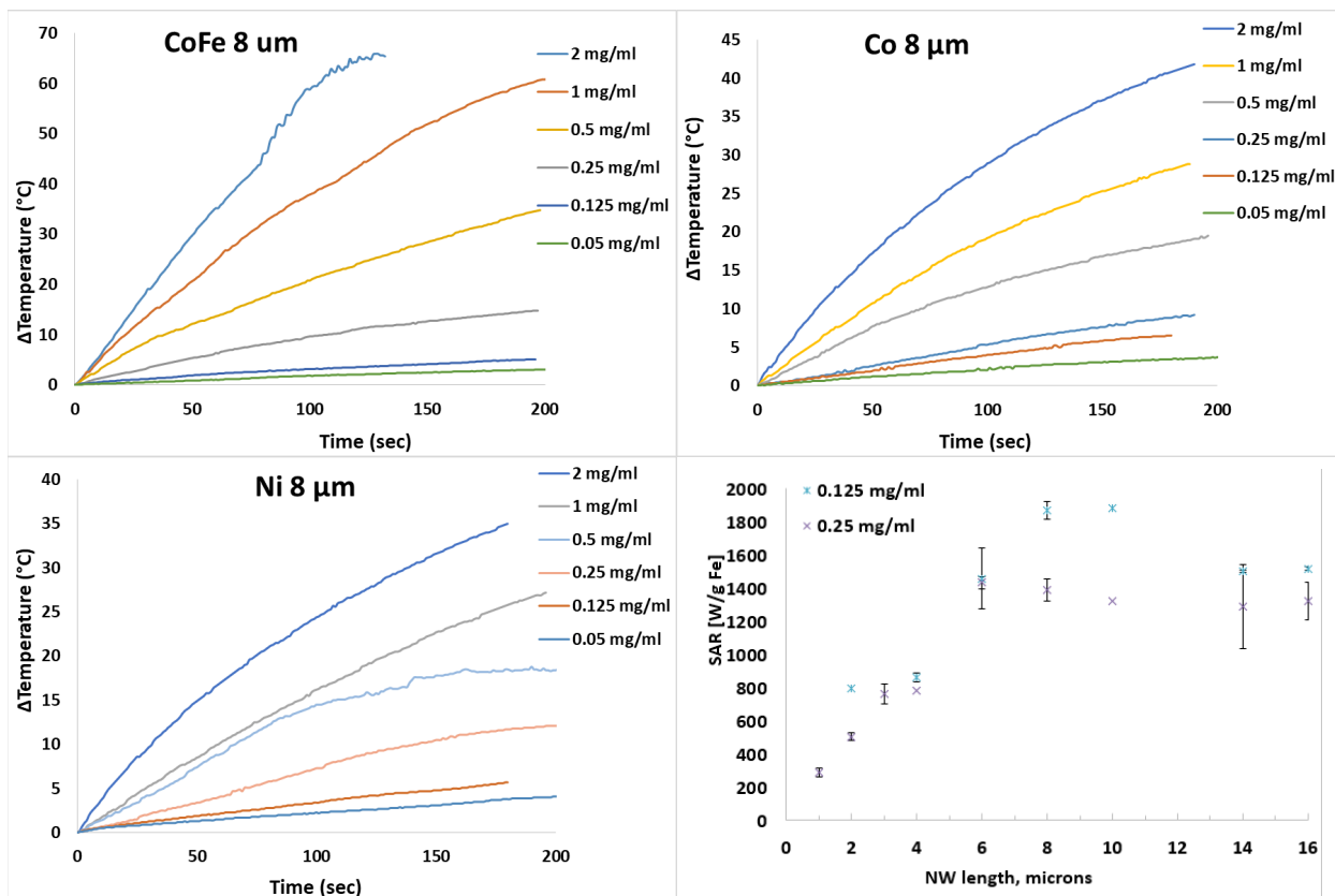
Figure S4. Temperature curves for 8 \mu m CoFe, Co, and Ni nanowires in glycerol at different concentrations. SAR values for different length CoFe nanowires in glycerol at various concentrations
