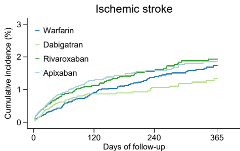
S1 Fig. Cumulative incidence of effectiveness outcomes Cumulative incidence of effectiveness outcomes associated with use of oral anticoagulants for non-valvular atrial fibrillation during one year of follow-up in Norway between 15 July 2013 and 31 December 2015. TIA, transient ischemic attack.
