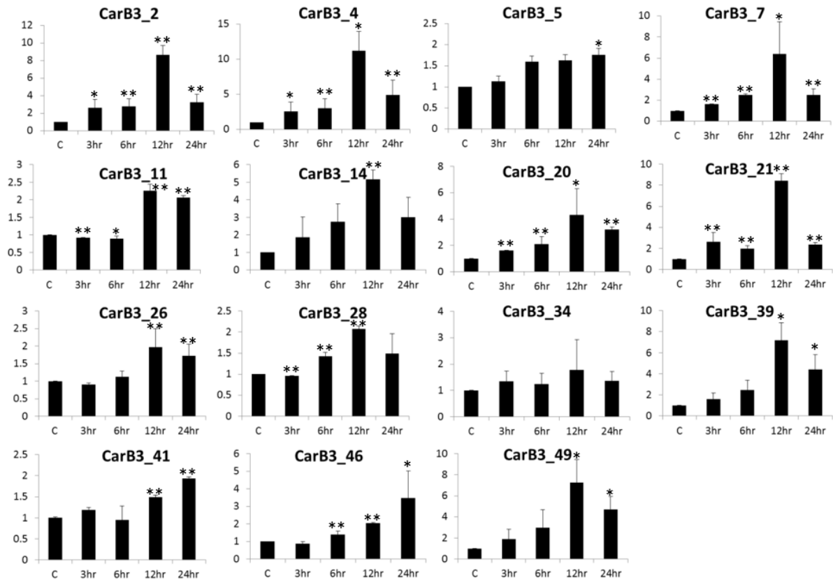
Online Resource 10: Expression analysis of 15 selected CarB3 genes in response to ABA (100 \mu M) treatment at different time points through qRT-PCR. Values on Y-axis denote relative expression values. Error bars indicate standard deviation ( \pm SD) of three biological replicates each calculated from three technical replicates. Asterisks indicate significant difference between control and other treated samples (t test, *P<0.05, **P<0.01).
