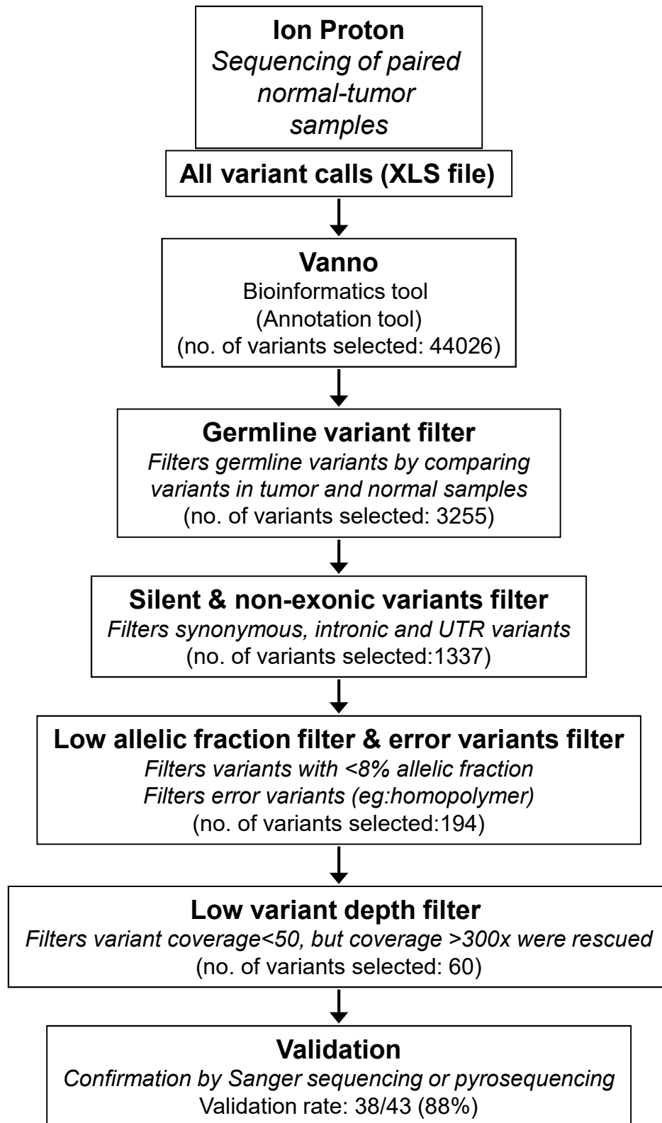
Fig. S1. Flow chart showing the step-wise analysis of our next-generation sequencing data.
