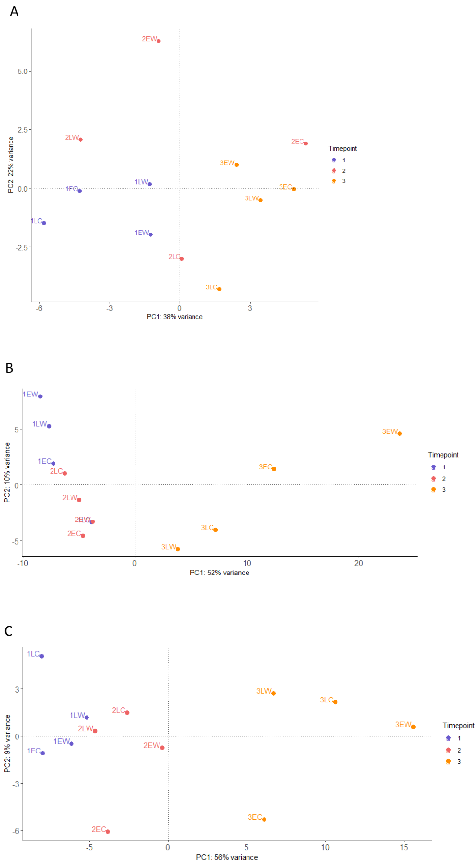
Fig S1. Clustering of samples based on principal component analysis (PCA). Samples collected from warm (W) and cold (C) temperature treatments from two different lines, early (E) and late (L), from three different time points and from three different tissues: a. hypothalamus, b. liver and c. ovary.
