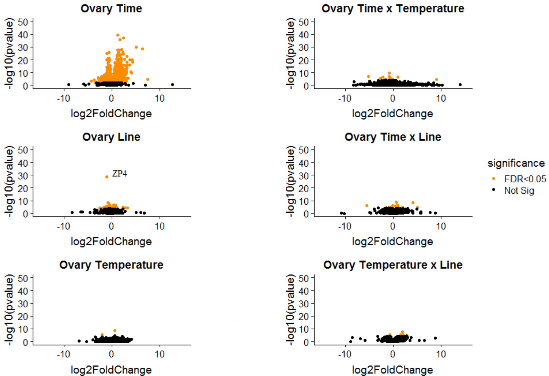
Fig S4. Volcano plots of all the transcripts analysed in ovary RNA-seq in six different models. Genes differentially expressed with p < 0.05 after correcting for false discovery rate are in orange. Genes with a p > 0.05 after correcting for false discovery rate are in black.
