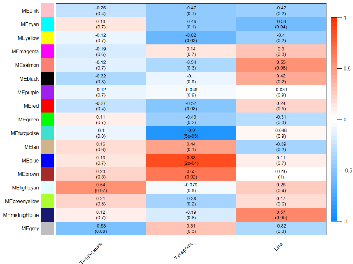
Fig S14. Matrix with the module-treatment relationships and corresponding p-values between the detected modules on the y-axis and treatments on the x-axis based on ovary RNA-seq. The relationships are coloured based on their correlation: red is a strong positive correlation, while blue is a strong negative correlation. The value at the top of each square represents the correlation coefficient between the module eigengene and the treatment with the correlation p-value in parentheses.
