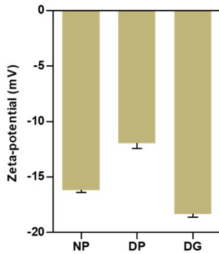
Figure S1. Zeta potential measurements of normal tooth protein (NP), dephosphorylated protein (DP) and deglycosylated protein (DG). The data represent the mean \pm standard error of three repeats.
