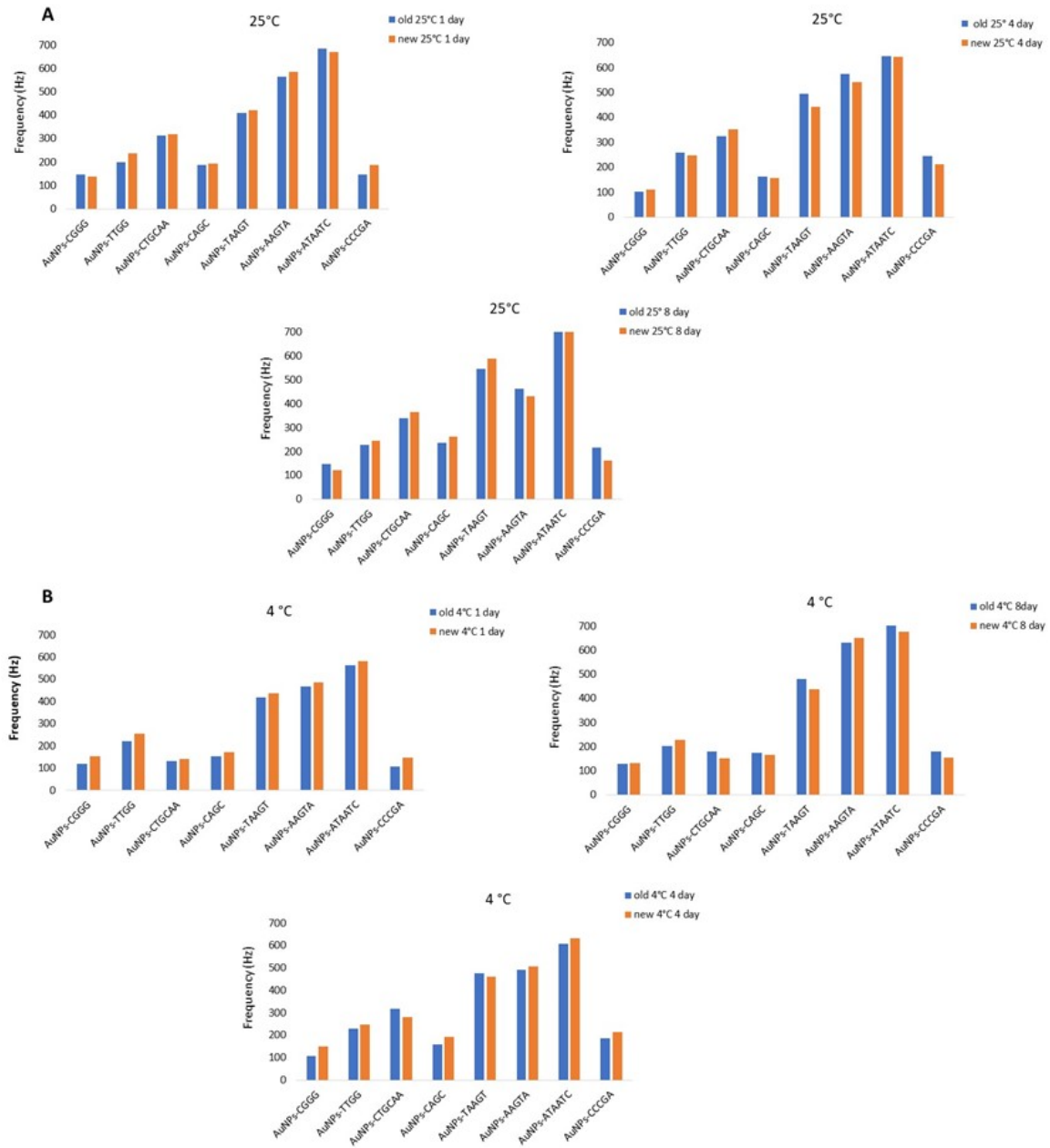
Figure S1. hpDNA-modified sensors array response vs. Octanal after three months from start analysis. (A) Represented the measurements carried out at 25 °C from 1th day to 8th day; (B) measurements carried out at 4 °C from 1st day to 8th day.
