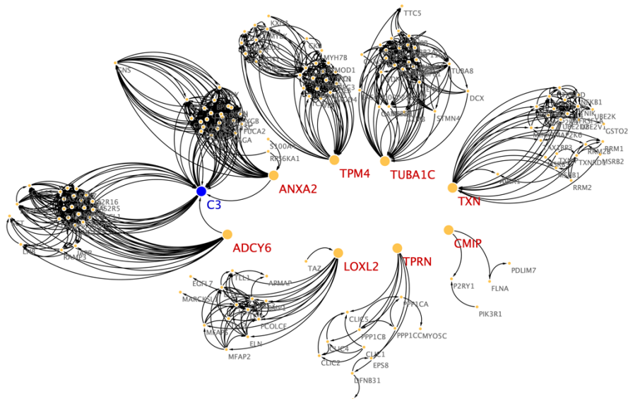
Figure S1. Protein-Protein network of TXN, ANXA2, TPM4, LOXL2, TPRN, ADCY6, TUBA1C and CMIP based on the STRING website. Orange is 8 key gene, blue is the connecting ADCY6 and ANXA2 .
