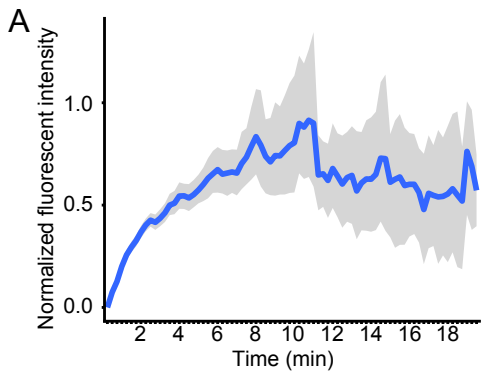
S3 Figure. Average and representative assembly and disassembly rates at FA.
