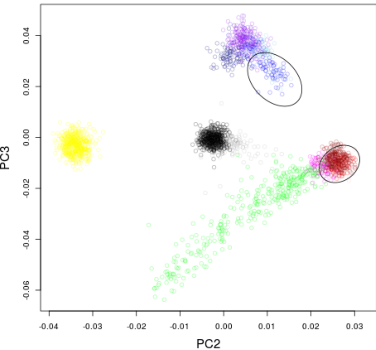
1000 Genomes, PC3 vs. PC2
