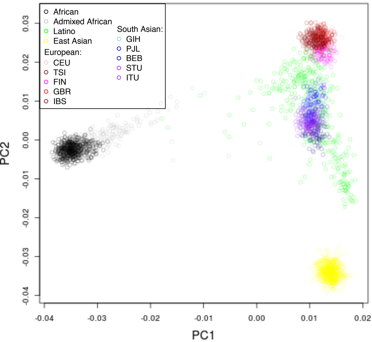
1000 Genomes, PC2 vs. PC1
