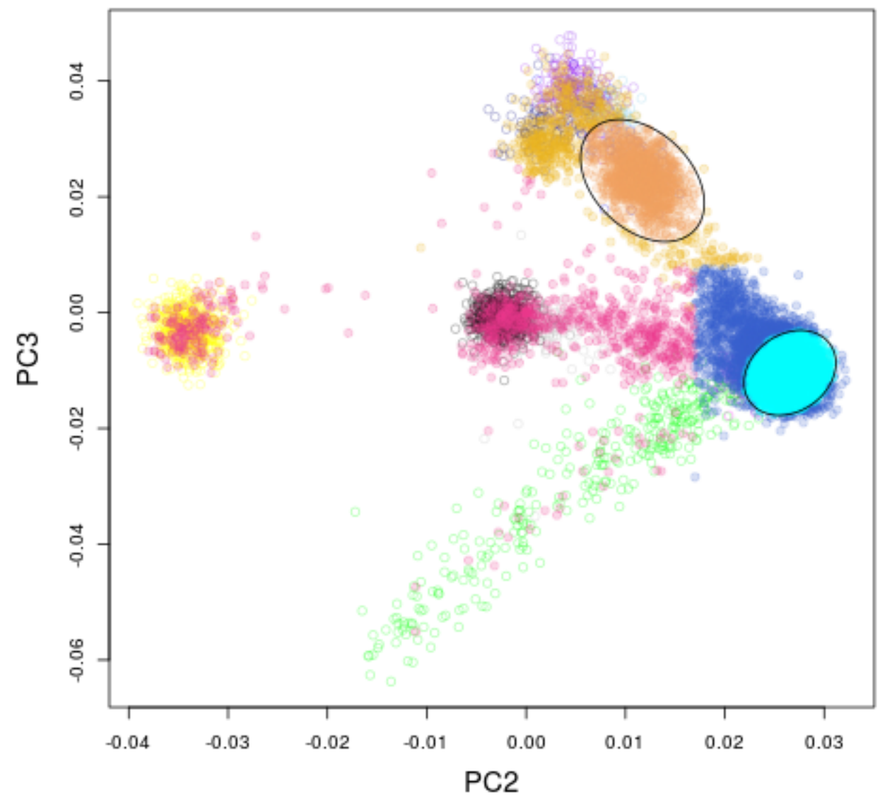
DDD projected onto 1000 Genomes, PC3 vs. PC2
