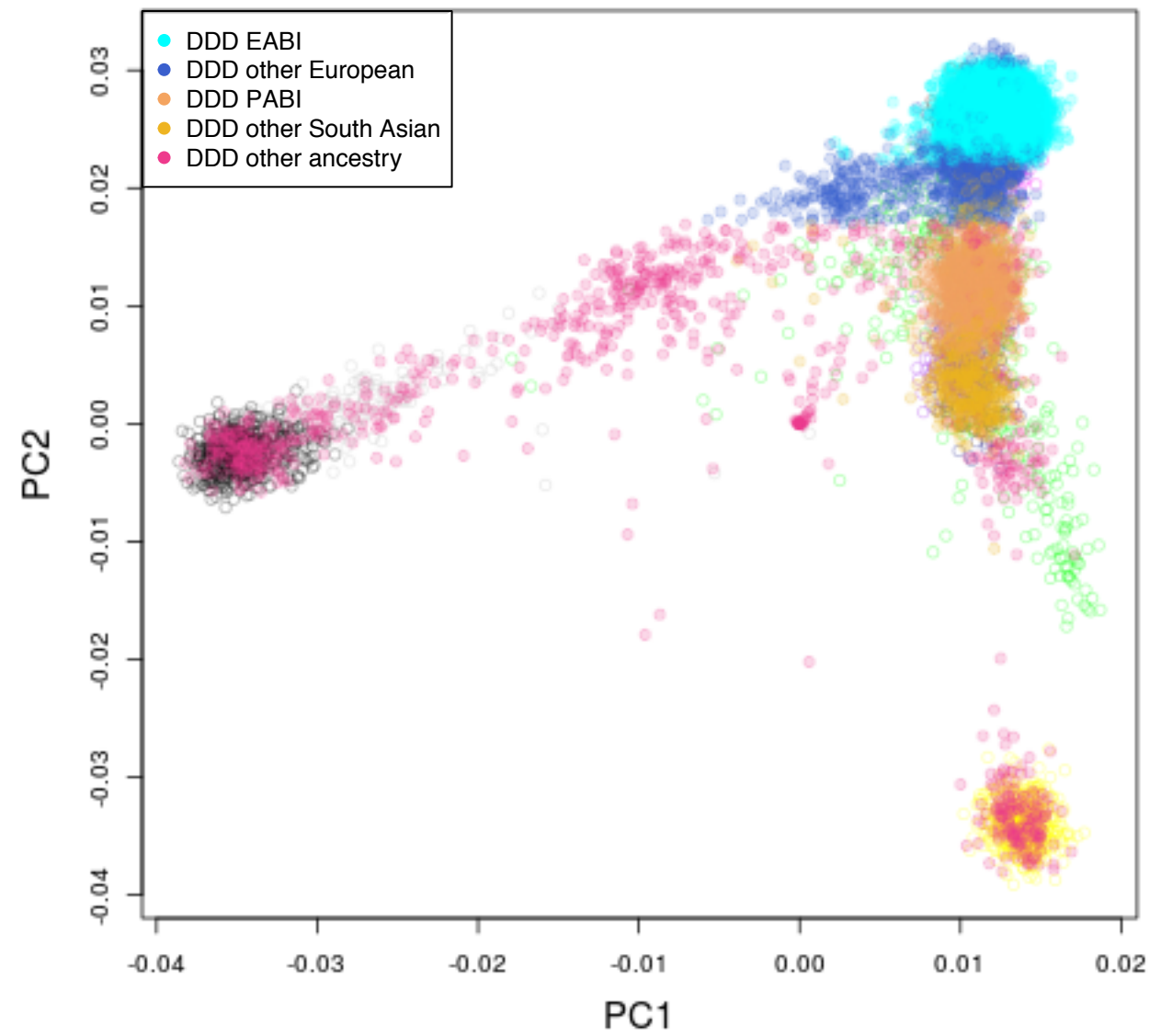
DDD projected onto 1000 Genomes, PC2 vs. PC1
