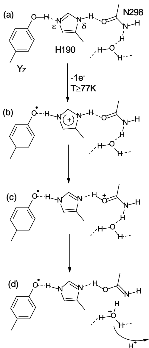
Scheme S1. Schematic illustration of the suggested deprotonation events which lead to proton exit after tyrosine oxidation in the S_2 state. (a) Y_z /His190/Asn298 prior to electron transfer. Oxidation of Y_z by P_{680}^+ initially leads to a state which is characterized by the wide EPR signal (b), followed by one characterized by the narrow EPR signal (c). Finally, one proton is expelled via a mechanism that involves amide to imidic acid tautomerism (d).
