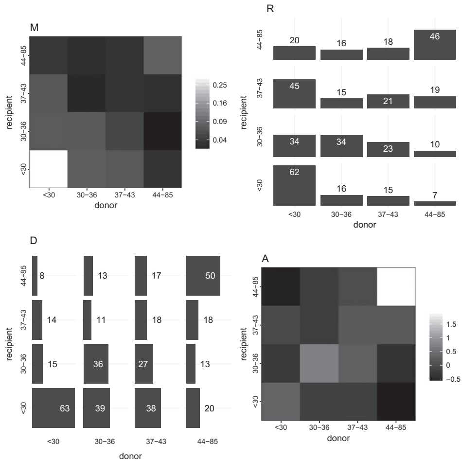
SUPPLEMENTARY FIG. S3. Patterns of transmission of HIV-1 subtype CRF02AG by age. See reading notes from Figure 1 in the main text.
