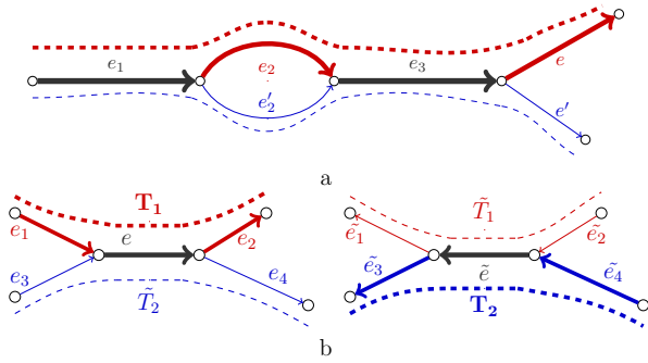
Figure 6. Using coverage depth for isoform reconstruction. Line width represents conventional and strand-specific coverage depths in figures (a) and (b) respectively. (a) Two isoforms of the same gene (red and blue dashed lines) have different expression levels and thus can be resolved using coverage depth. (b) Two transcripts T_1 and T_2 (red and blue bold dashed lines respectively) share a reverse-complement sequence and thus can be resolved using strand-specific reads.
