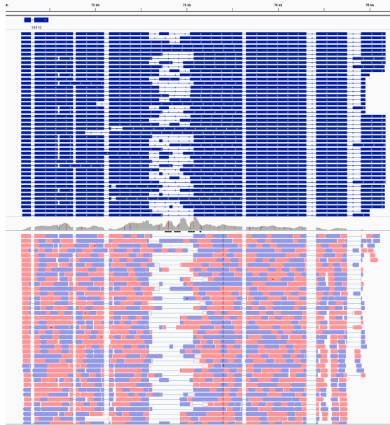
Jgi 10510
