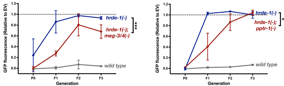
Figure 6. Mutants with Defective Germ Granules Inherit RNAi in the Absence of HRDE-1
